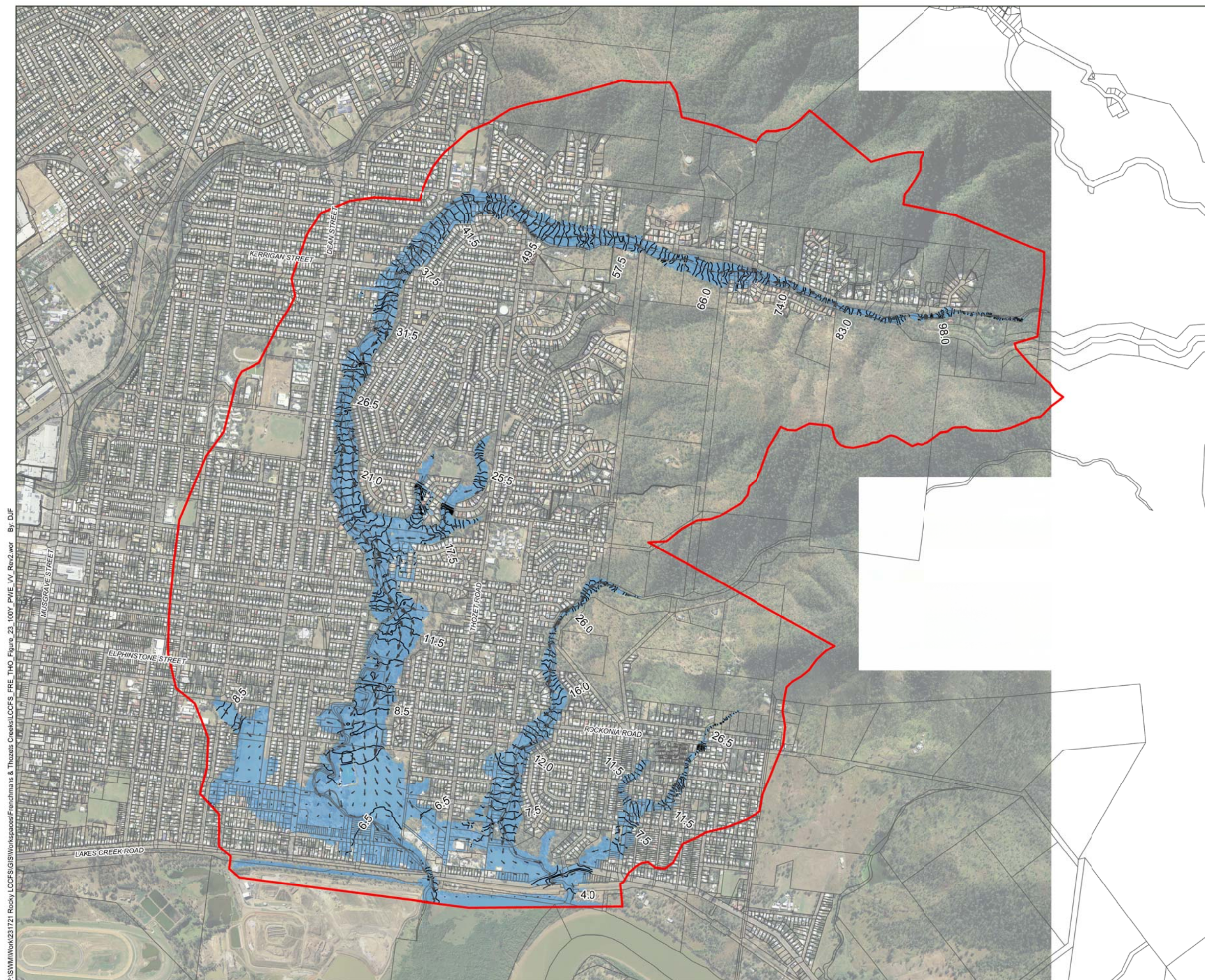
Figure 23: Existing Conditions - 100 Year ARI Inundation Extents, Peak Water Surface Elevations and Velocities
