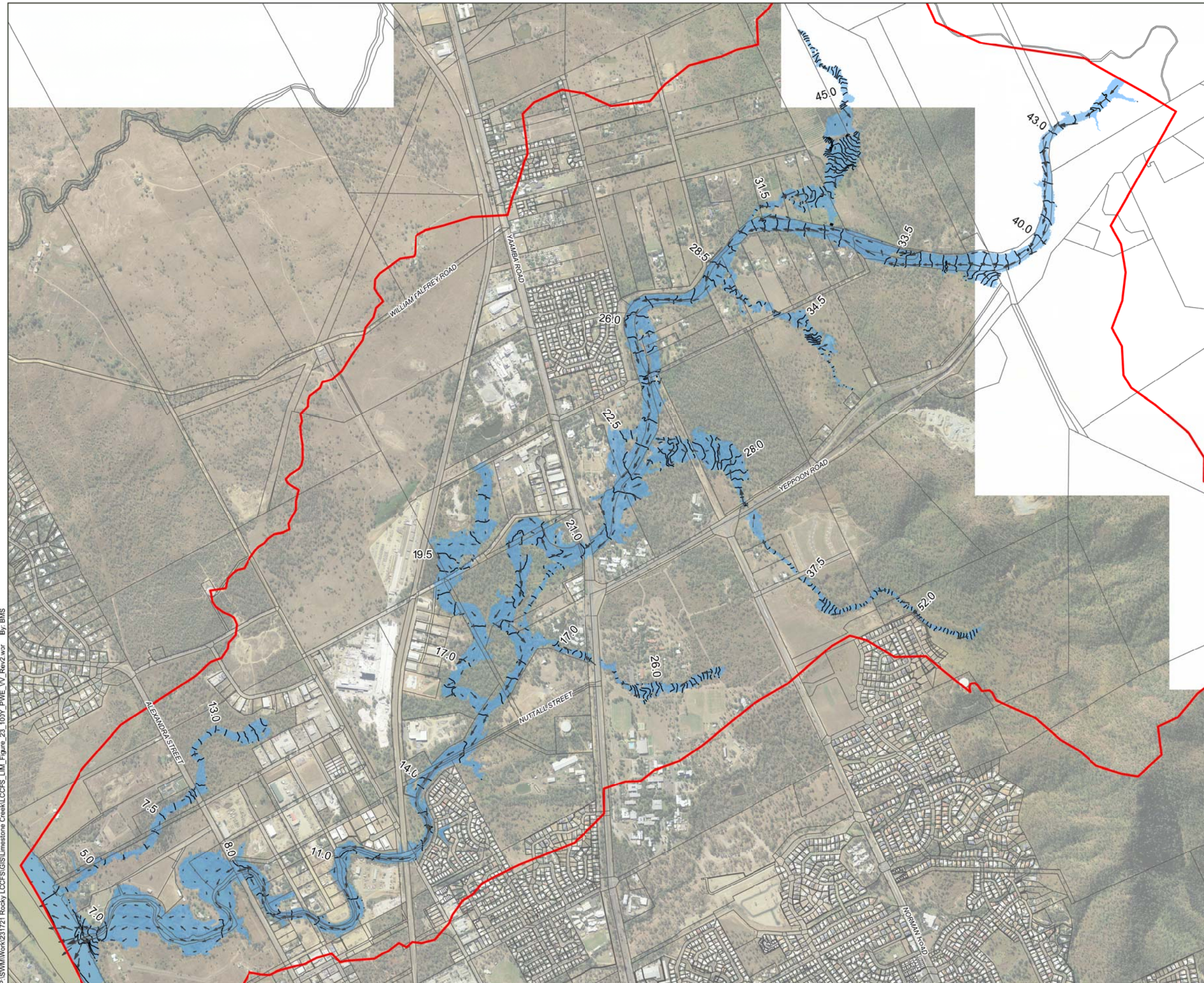
Local Creek Catchments Flood Study: Limestone Creek Figure 23: Existing Conditions - 100 Year ARI Inundation Extents, Peak Water Surface Elevations and Velocities
