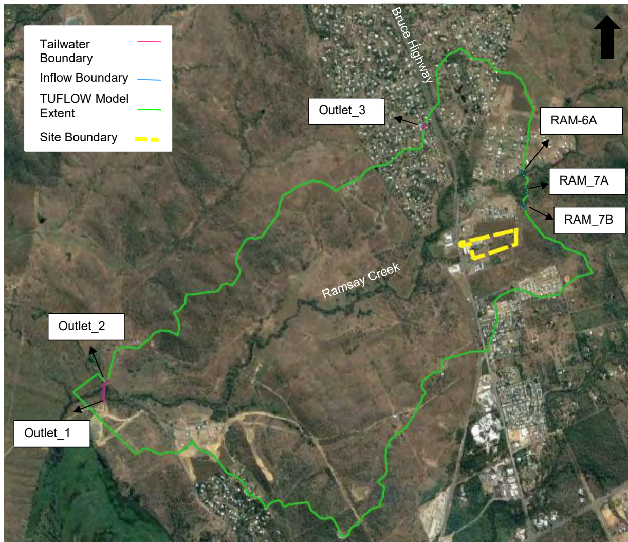
Figure 3-1: Model Boundary Conditions
