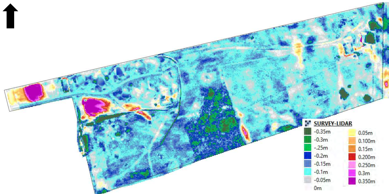
Figure 3-7: Lidar TIN - Natural TIN
