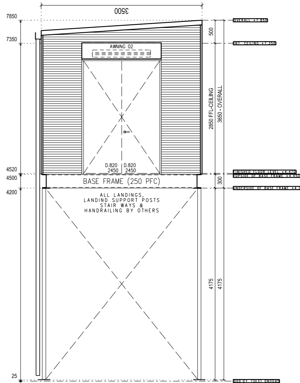
04 - EXTERNAL ELEVATION
