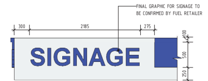
5 S4 - ILLUMINATED CANOPY SIGN - 3 OFF 1: 25
