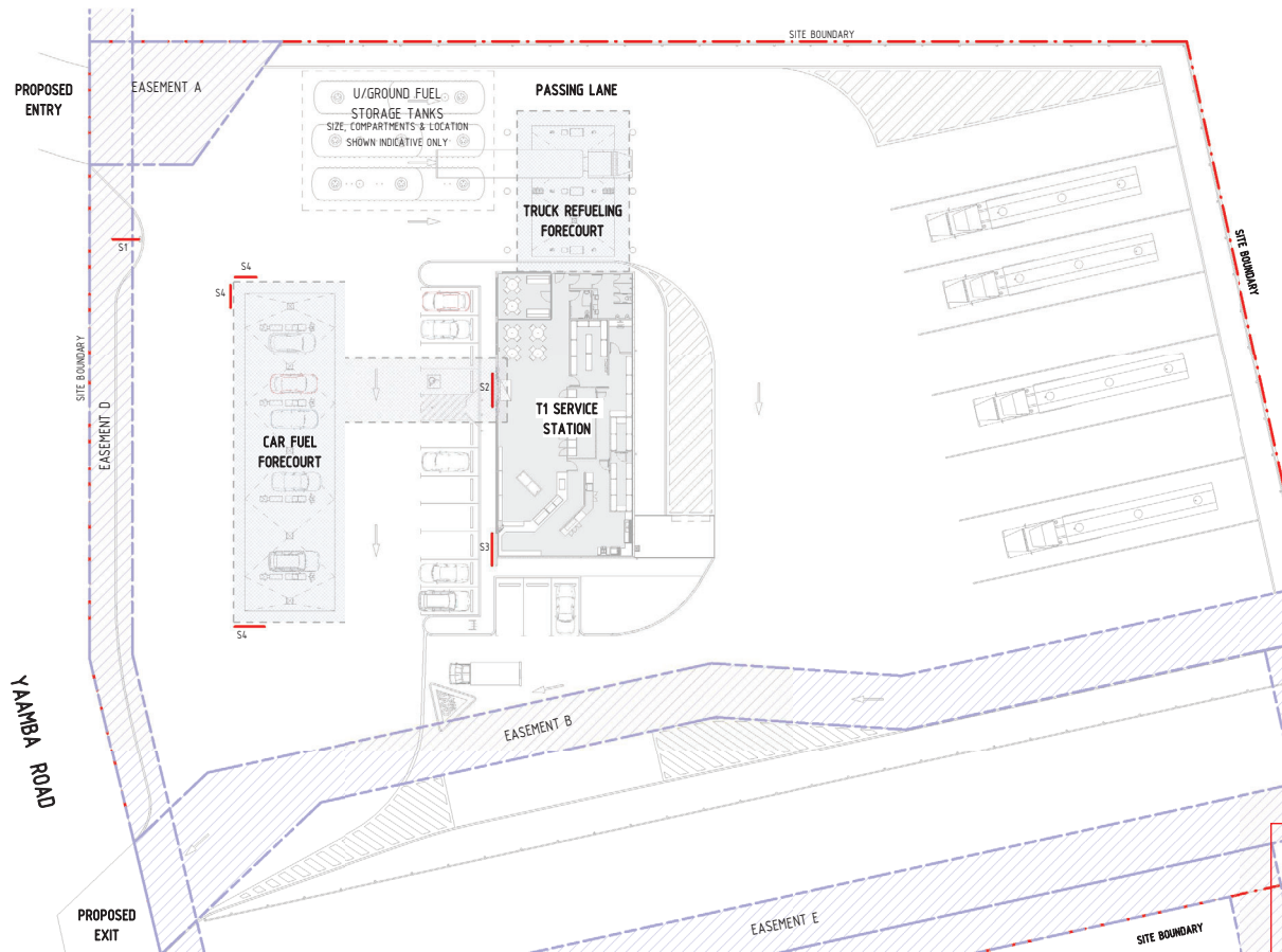
1 SIGNAGE PLAN 1: 250
