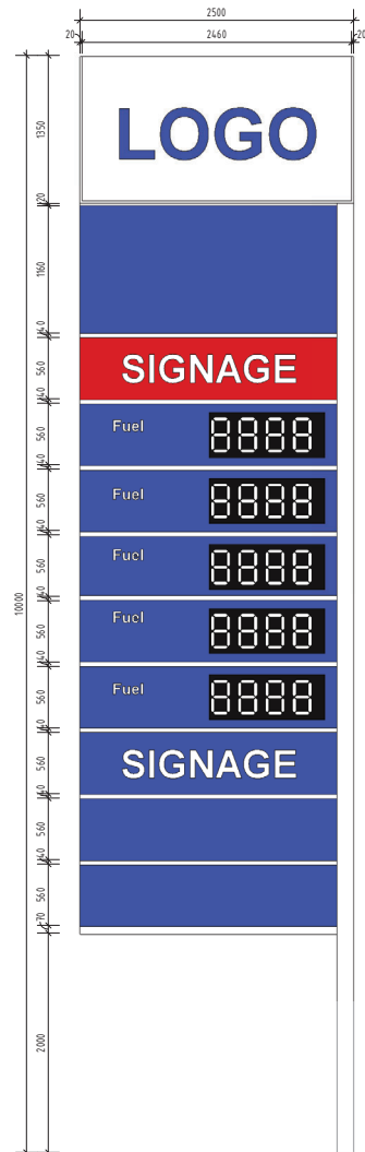
2 S1 - 10m ILLUMINATED PYLON SIGN - 1 OFF 1: 25
