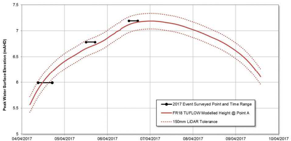
Figure 25 2017 Event Calibration – Point A
