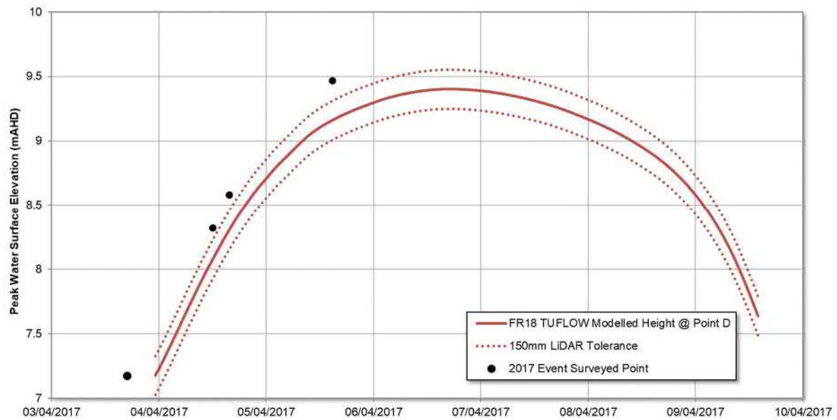
Figure 28 2017 Event Calibration – Point D
