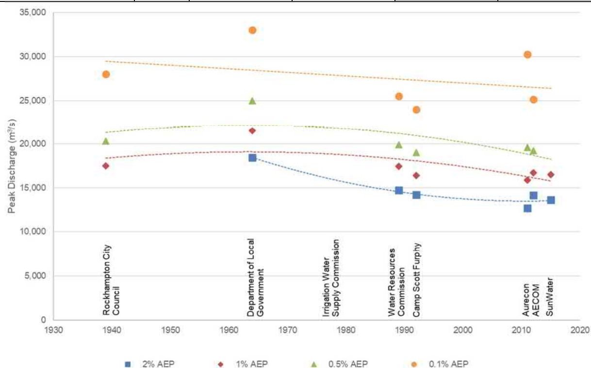
Figure 7 Timeline of FFA Results for Rockhampton
