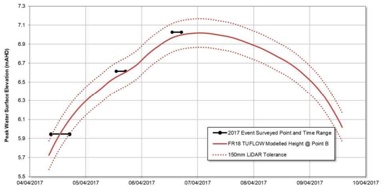
Figure 26 2017 Event Calibration – Point B
