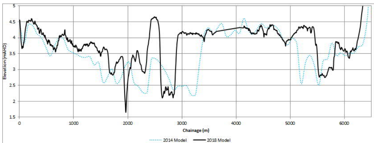
Figure 18 Downstream 1-D Network Cross Section Comparison (CH280)
