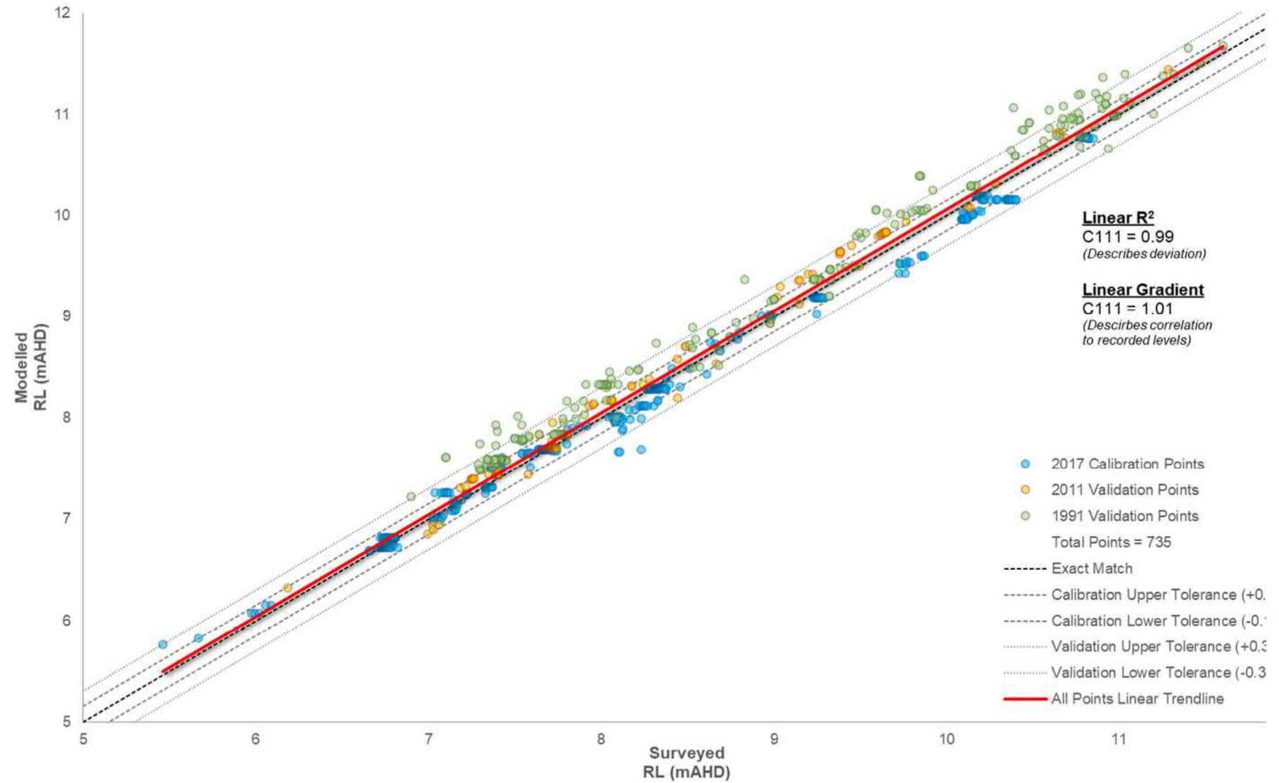
Figure 48 Full Dataset (735 points) Scatter Plot
