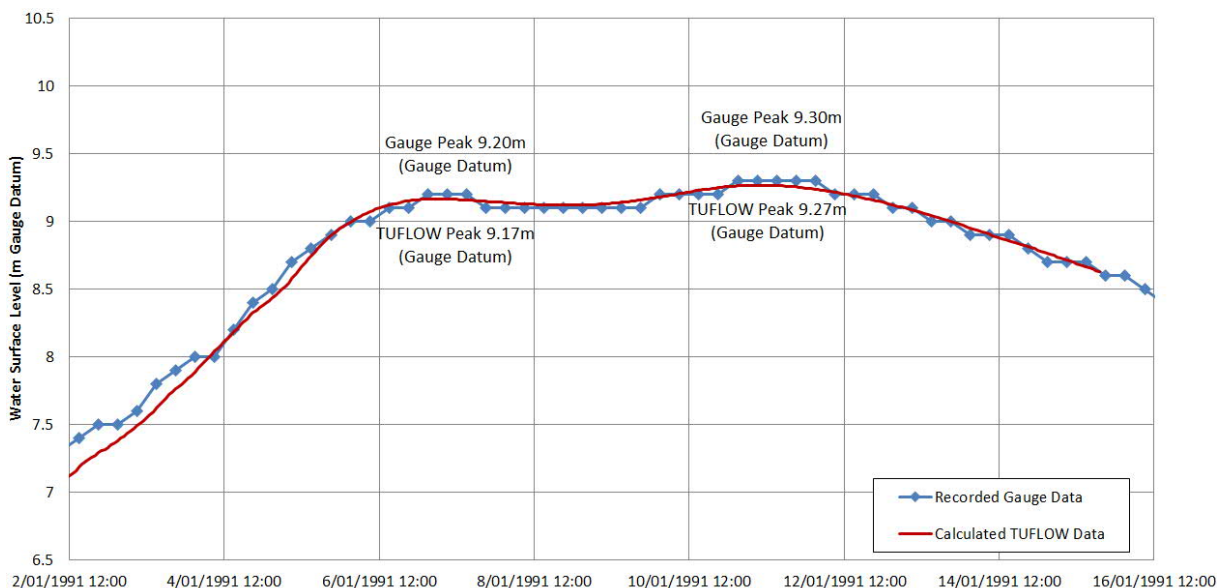
Figure 41 SRFL Rockhampton Flood Gauge Comparison – 1991 Event (source: AECOM, 2014)
