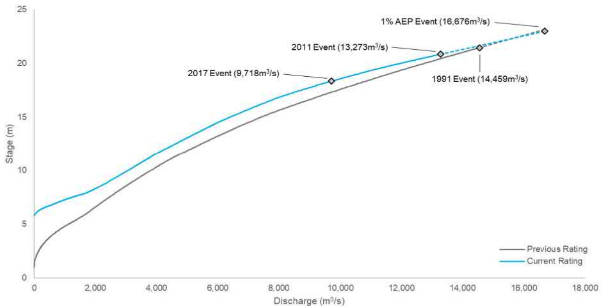
Figure 4 The Gap (130005A) Gauge Rating Curve Comparison
