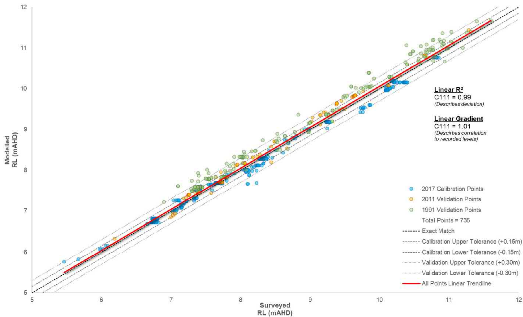
Figure E1 Full Dataset (735 points) Scatter Plot
