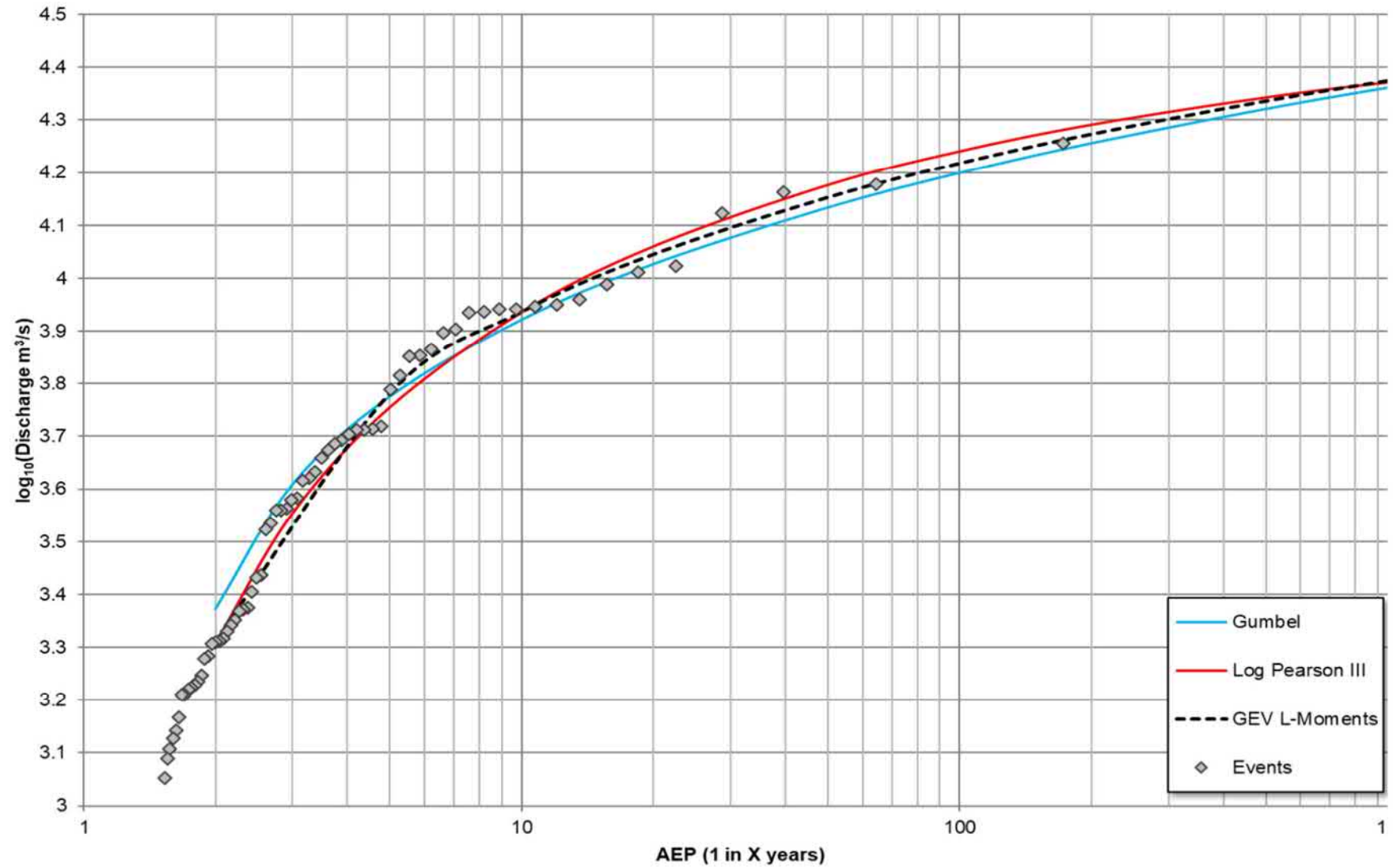
Figure 11 Comparison of Probability Models
