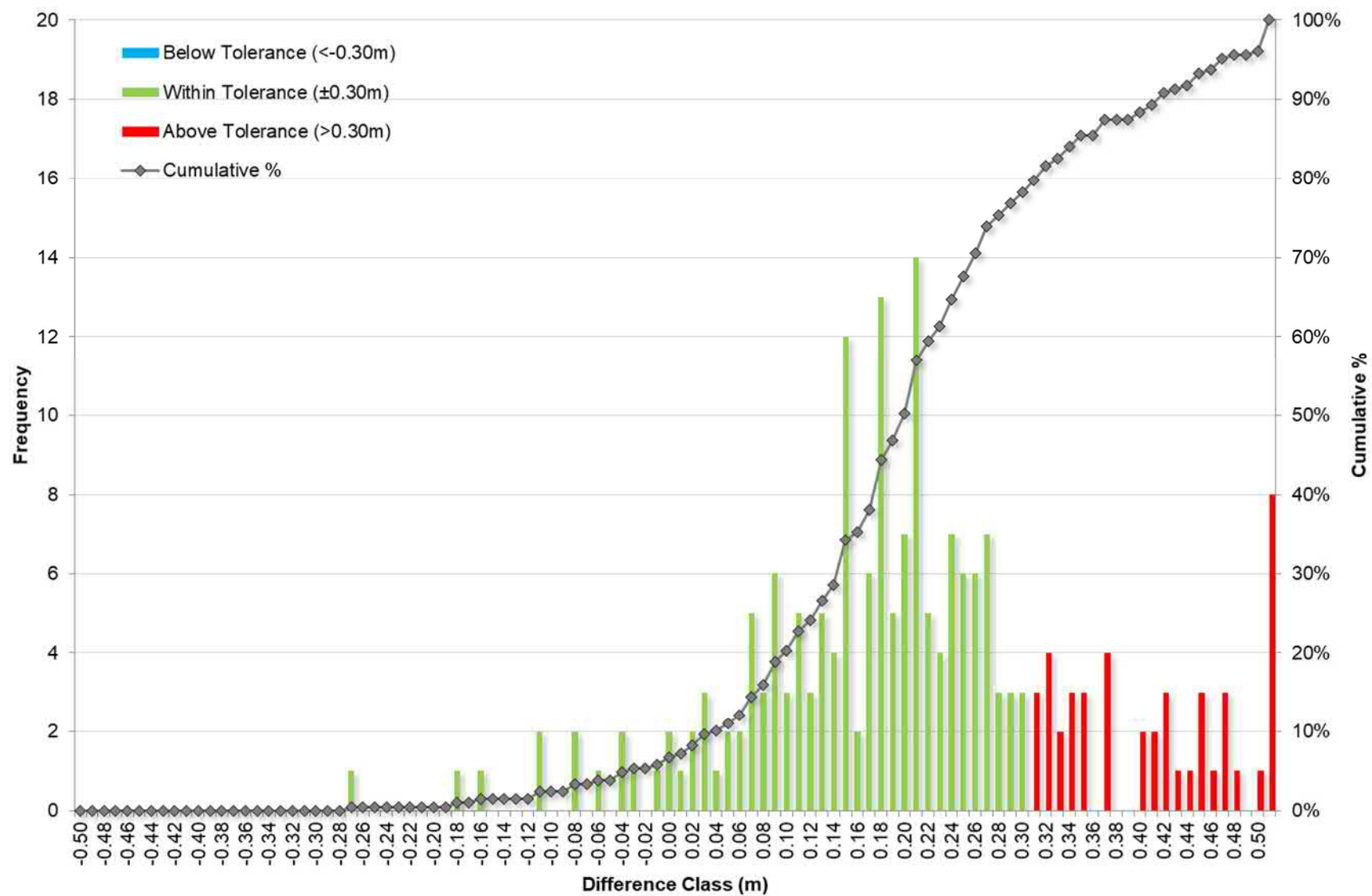
Figure 42 1991 Event Calibration Distribution
