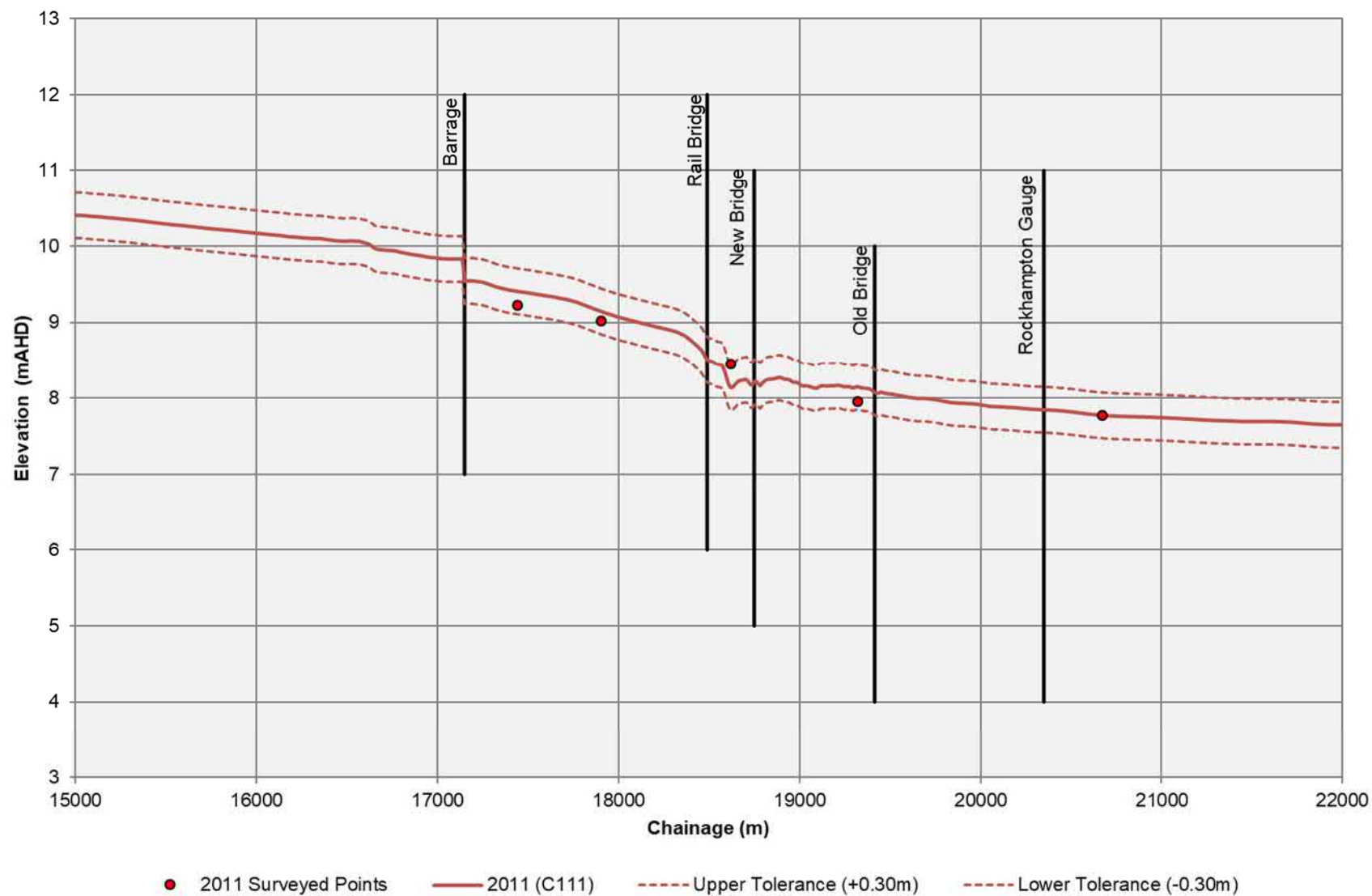
Figure 36 2011 Event Calibration – Long section Along Main River Channel
