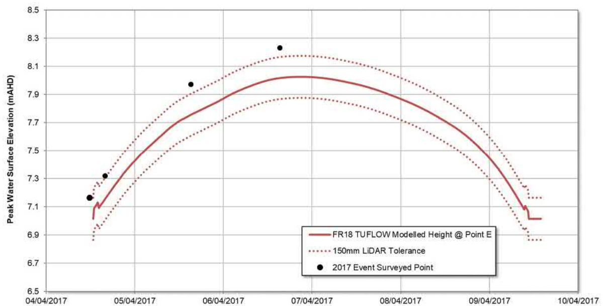
Figure 29 2017 Event Calibration – Point E
