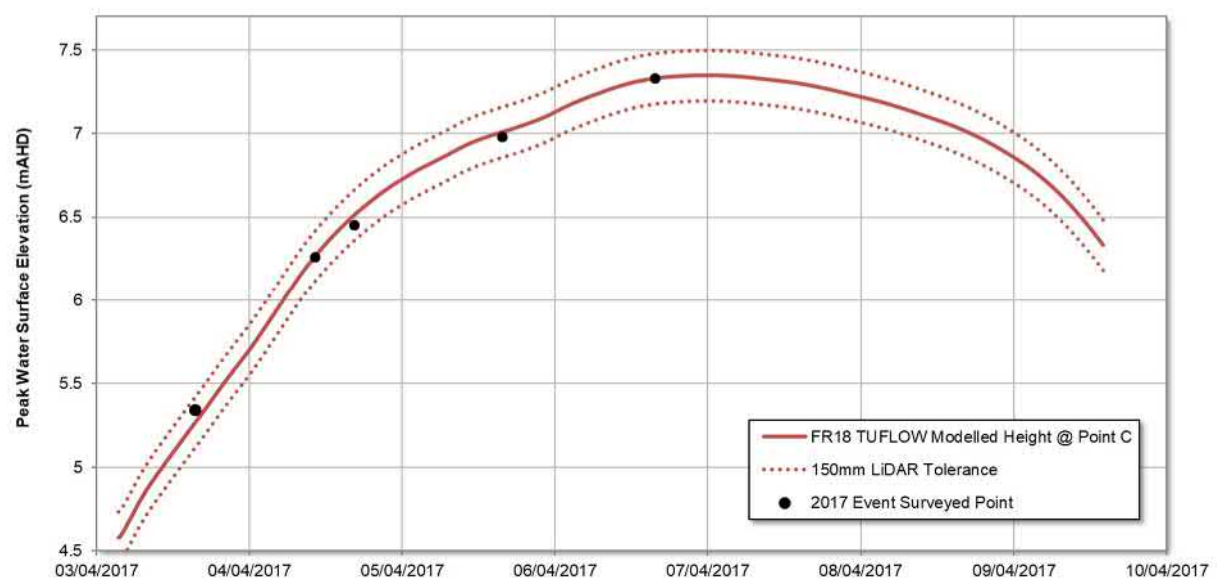
Figure 27 2017 Event Calibration – Point C
