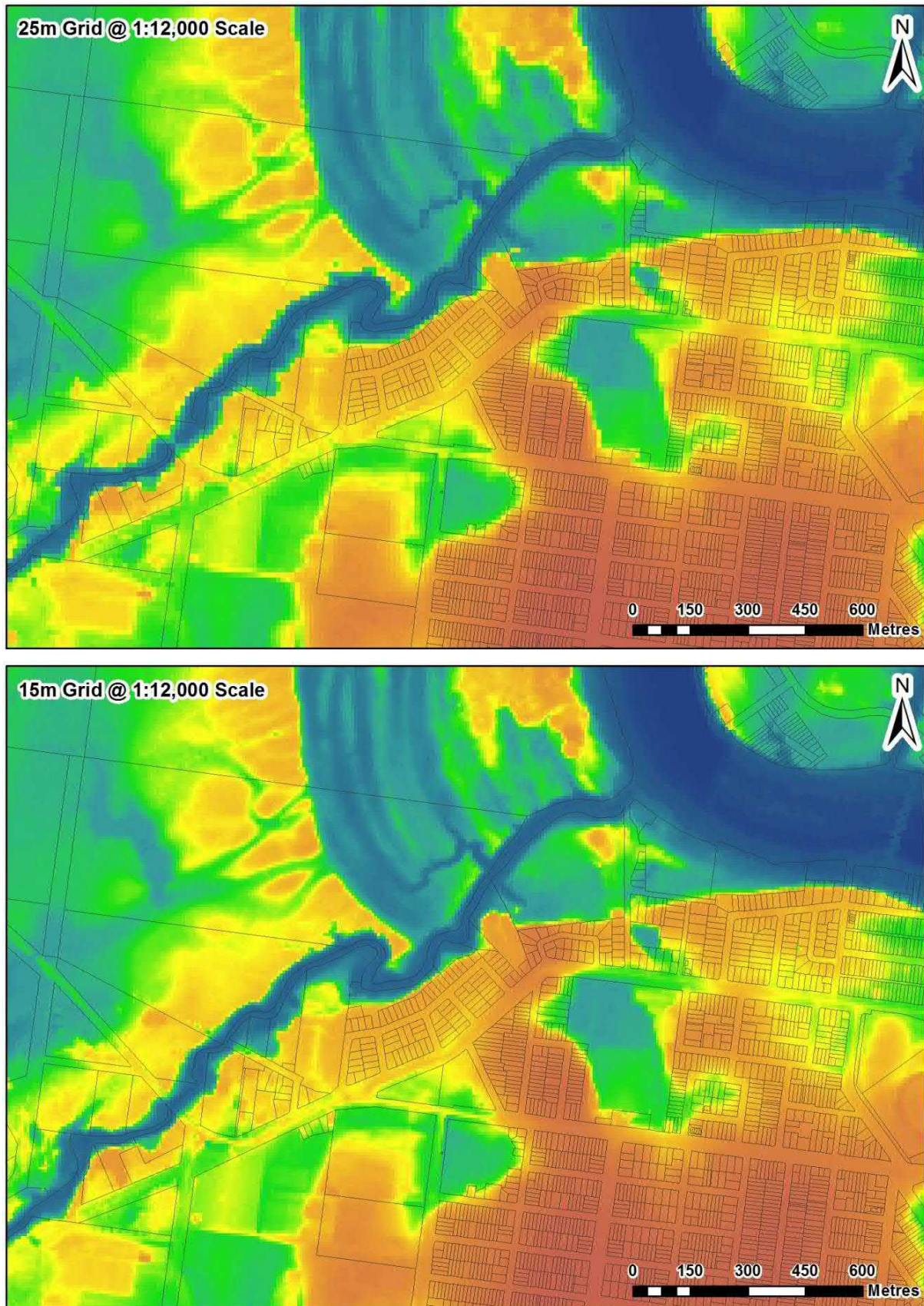
Figure 15 Comparison of Model Grid Cell Sizes -1:12000 Scale
