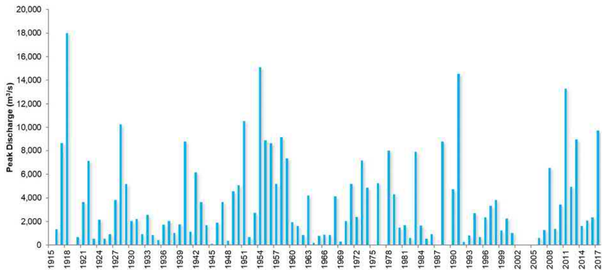
Figure 10 Annual maximum data series used in FFA update
