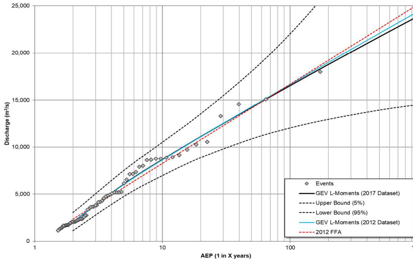
Figure 12 Adopted GEV (LH = 4) Distribution
