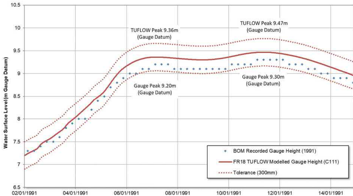
Figure 40 1991 Event Validation – Rockhampton Flood Gauge Comparison
