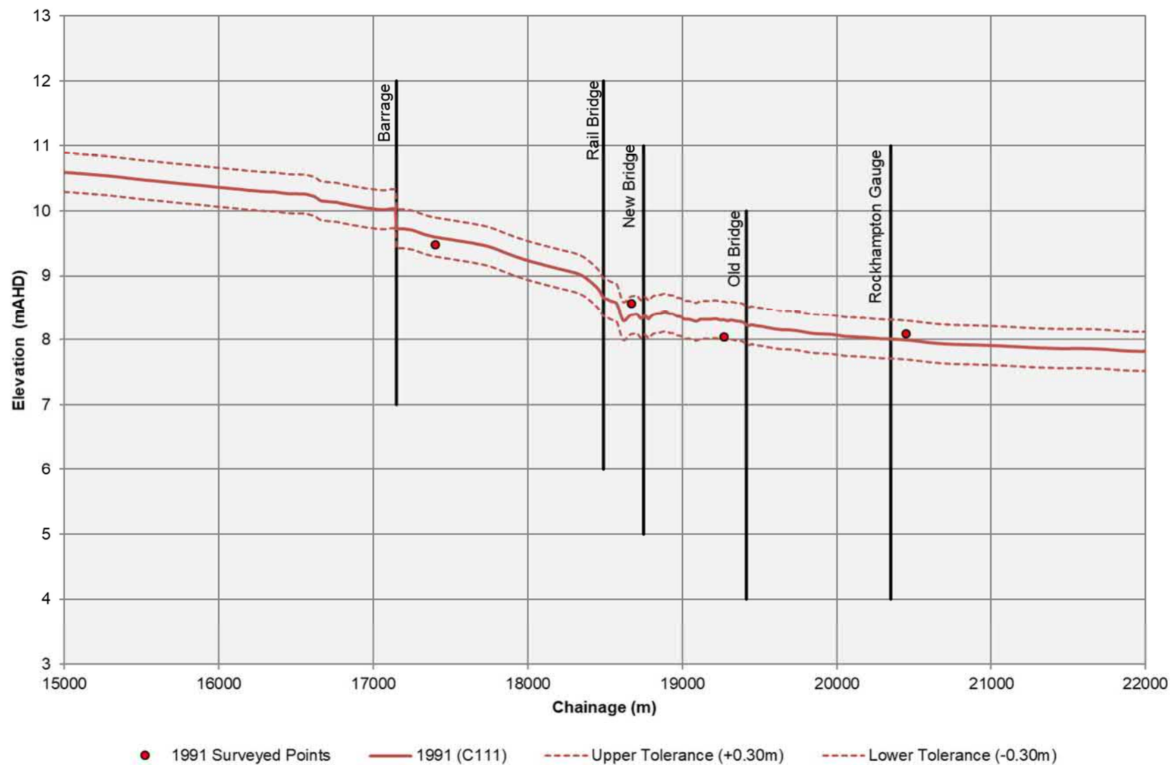
Figure 44 1991 Event Validation – Long section Along Main River Channel
