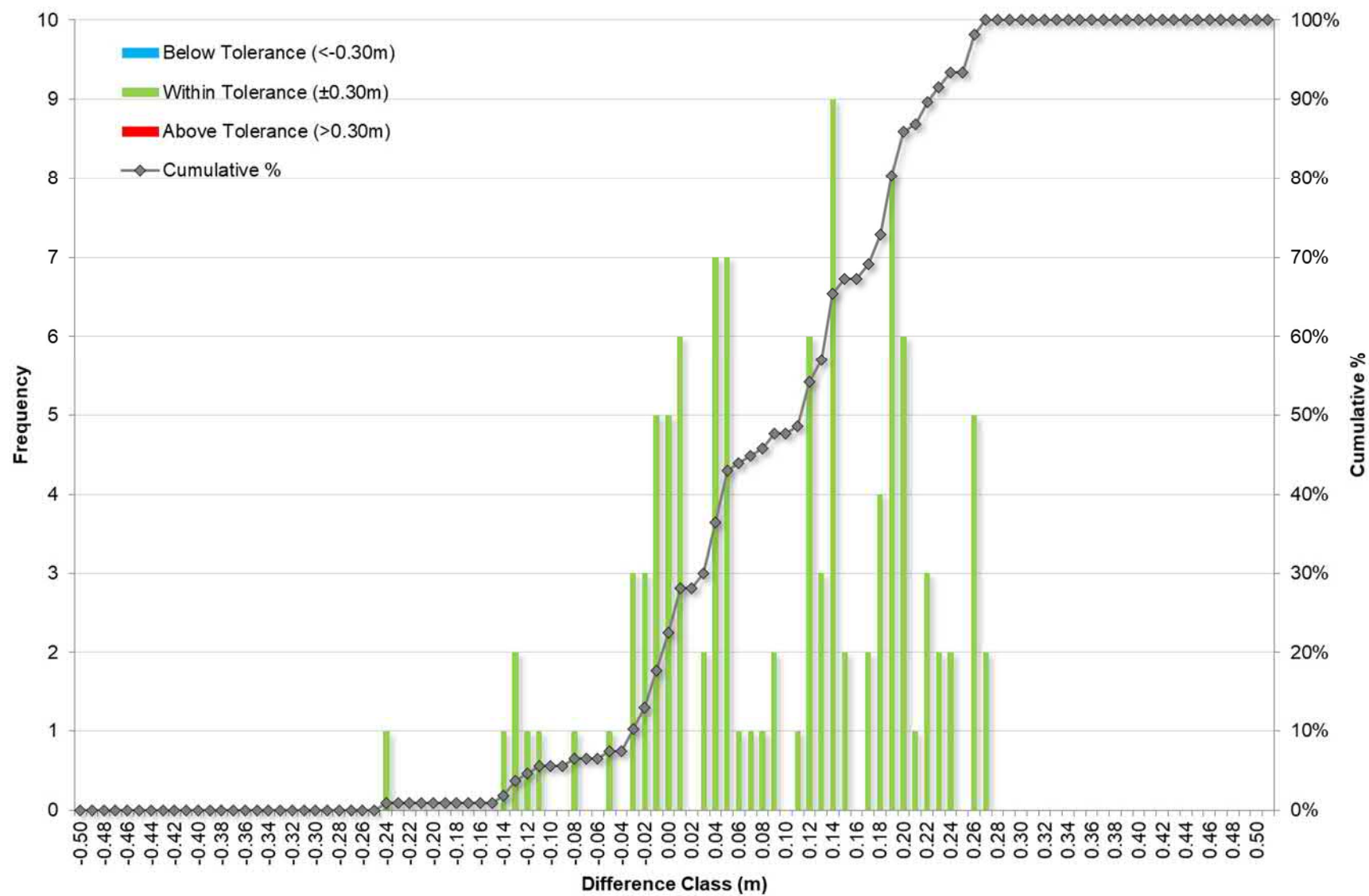
Figure 34 2011 Event Calibration Distribution
