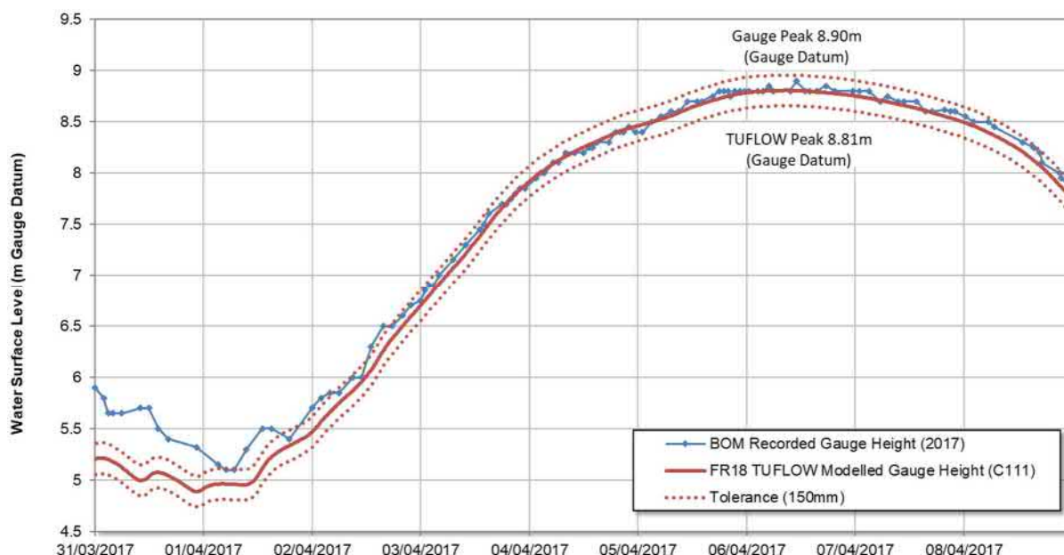
Figure 19 2017 Calibration Event – Rockhampton Flood Gauge Comparison
