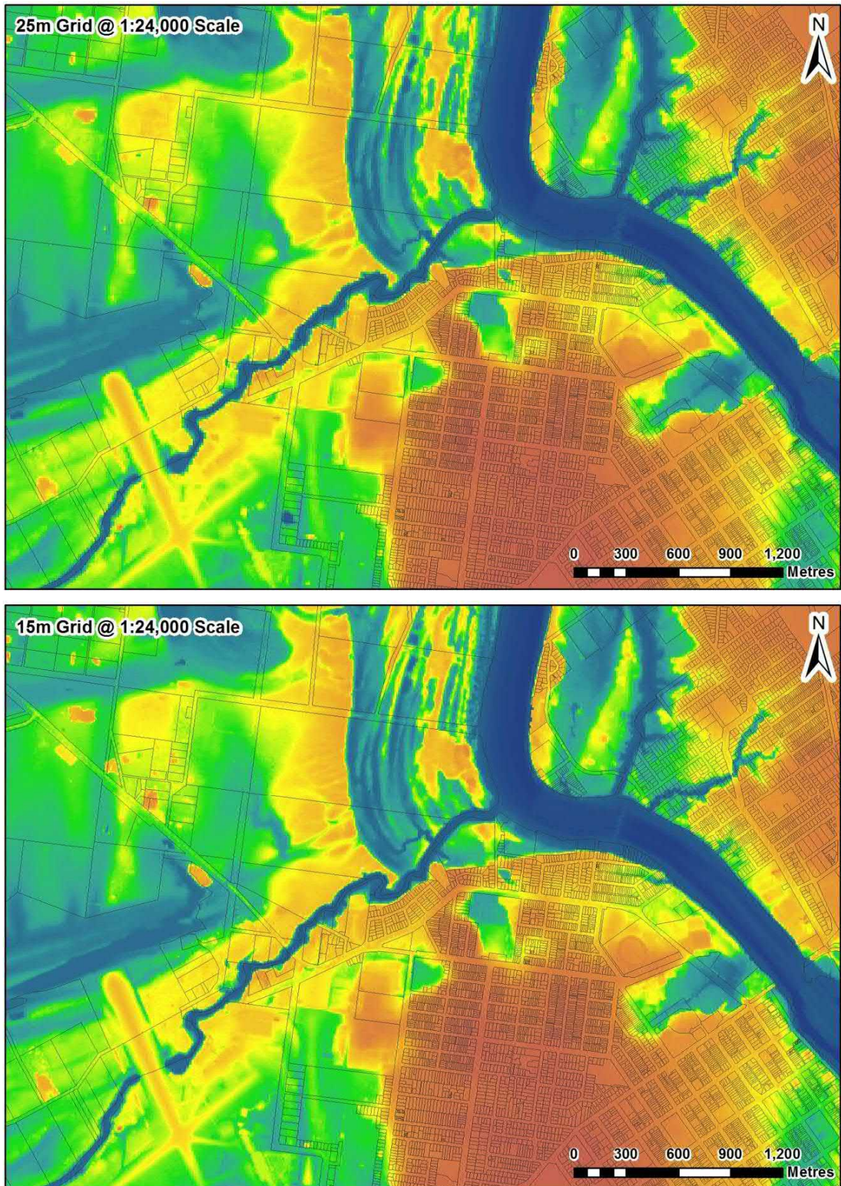
Figure 14 Comparison of Model Grid Cell Sizes -1:24000 Scale
