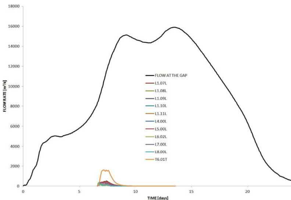
Figure 1 1% AEP Fitzroy River and Local Catchment Inflows (reproduced from FRFRPS Volume 3 report)
