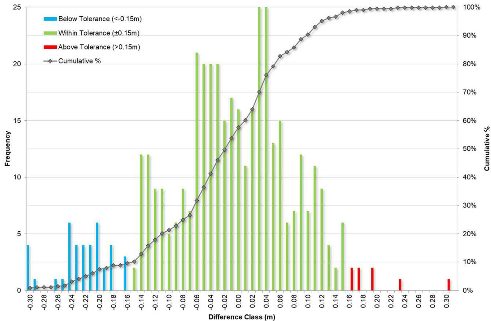
Figure 20 2017 Calibration Event Histogram
