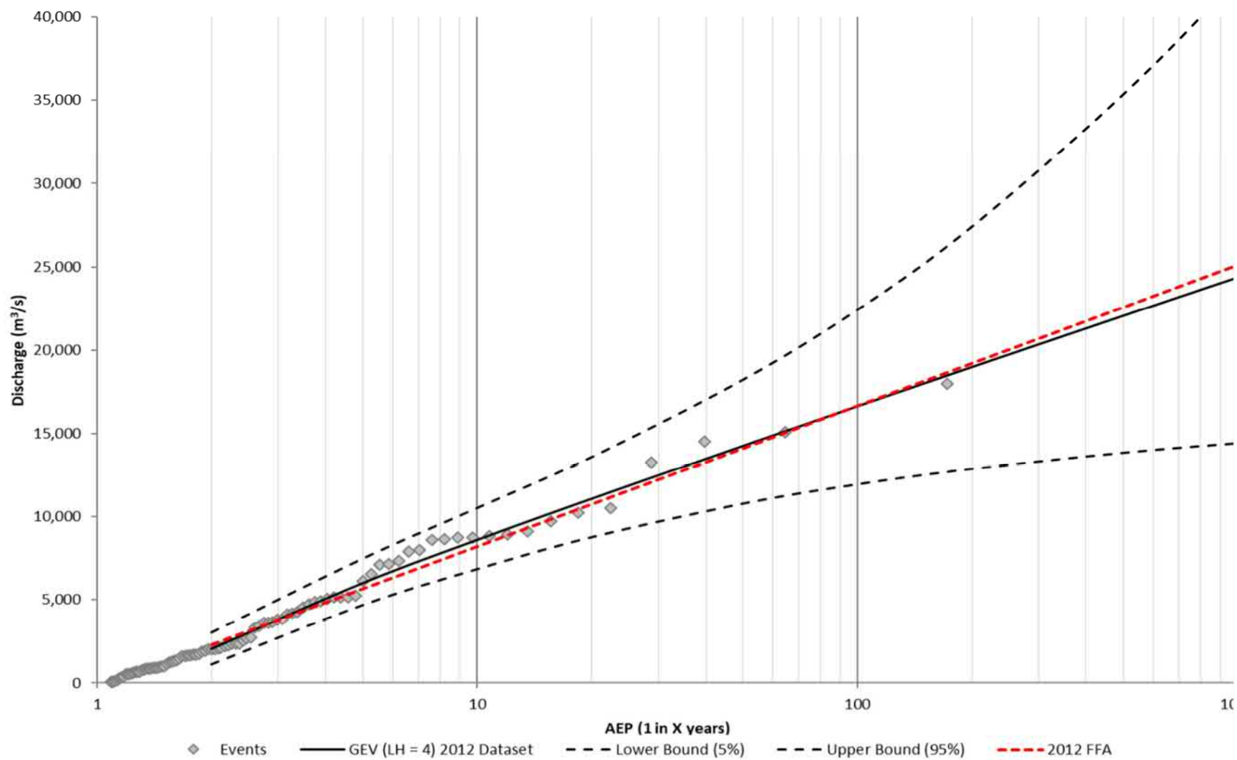
Figure 8 Adopted GEV (LH = 4) Distribution (2012 data)
