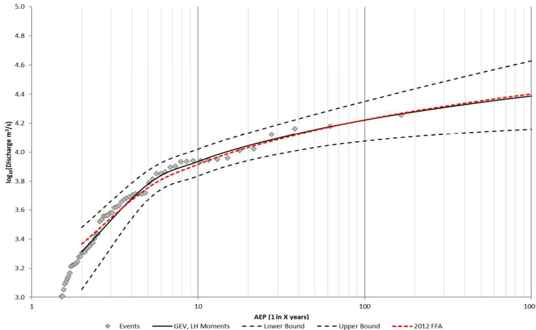
Figure 9 Adopted GEV (LH = 4) Distribution ( \log_{10} Vertical Scale)
