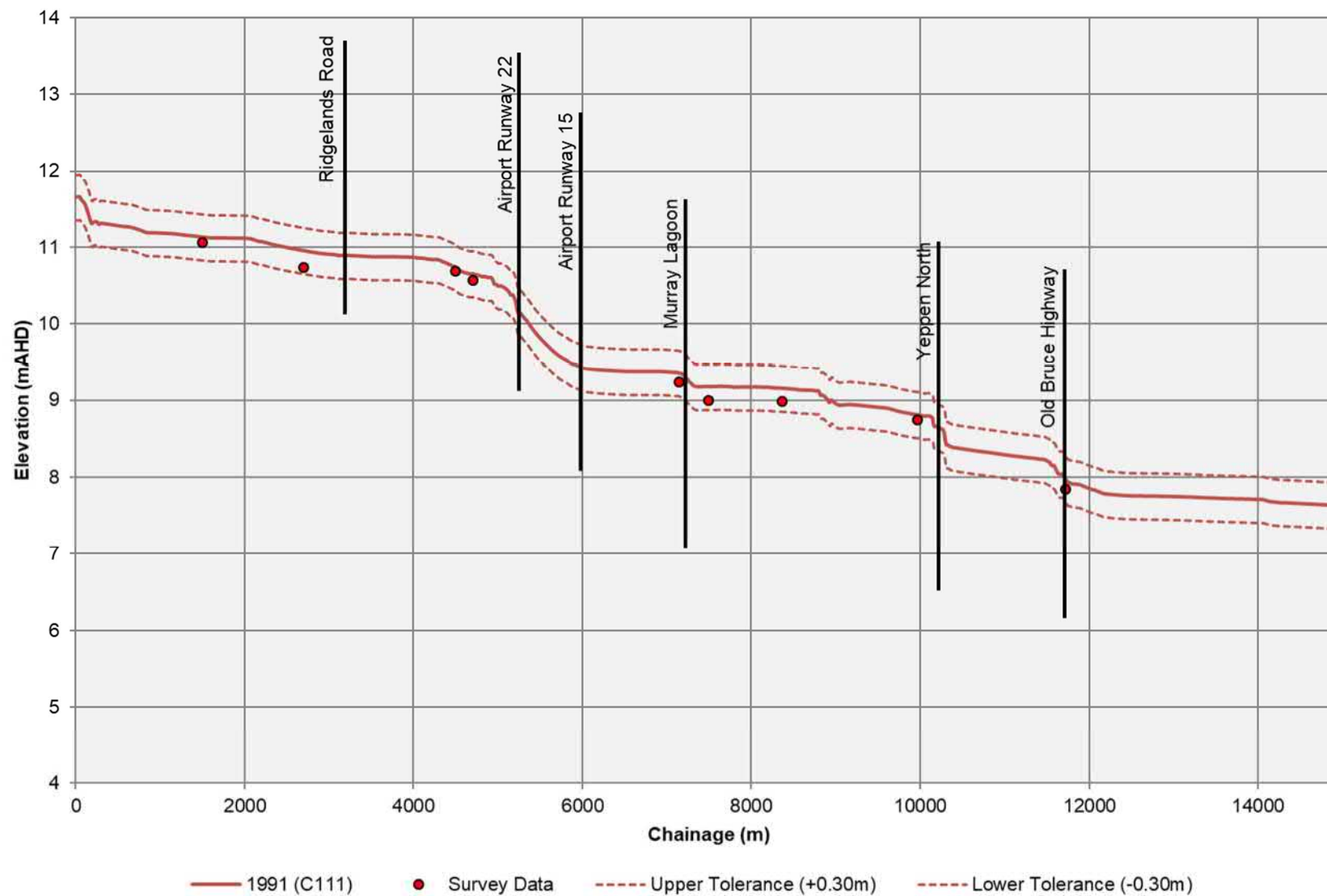
Figure 45 1991 Event Validation – Long section Along Western Floodplain
