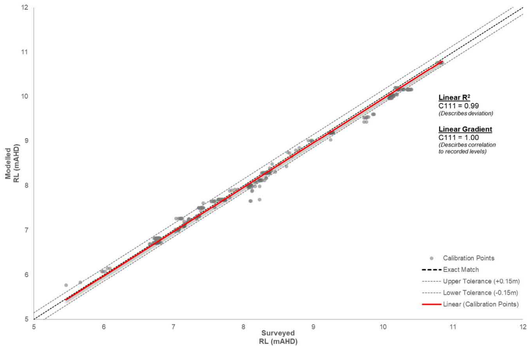
Figure 21 2017 Event Calibration Scatter Plot
