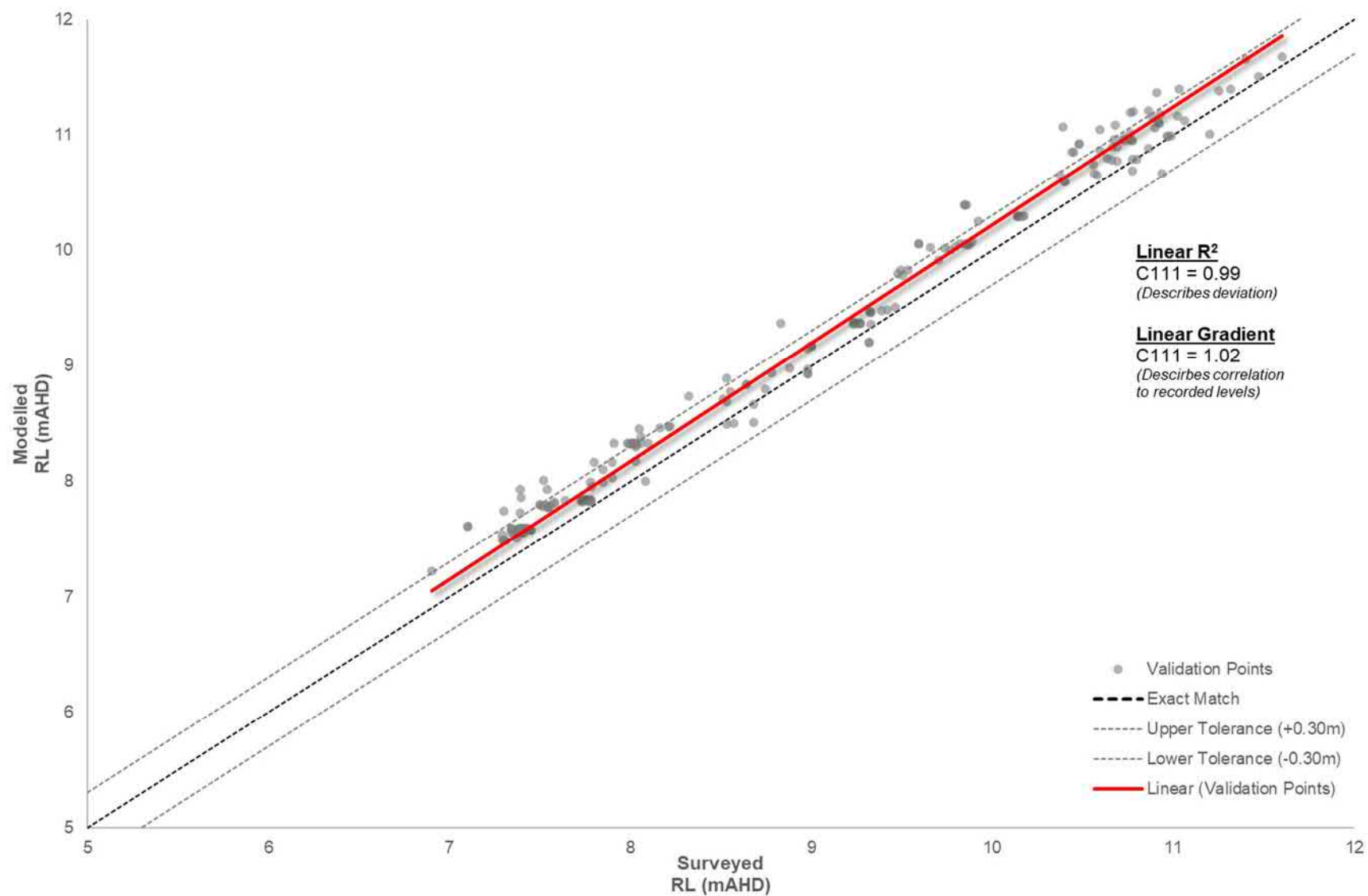
Figure 43 1991 Event Calibration Scatter Plot
