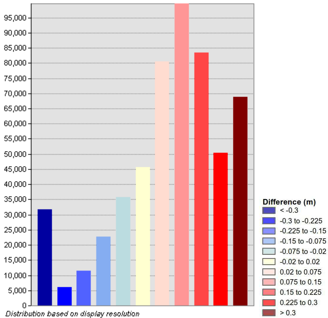
Figure 6 Histogram of Difference in LiDAR Datasets (2015/16 minus 2009)
