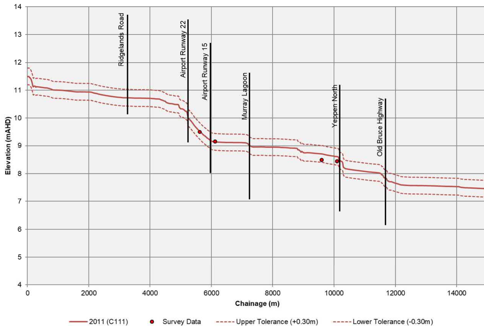
Figure 37 2011 Event Calibration – Long section Along Western Floodplain
