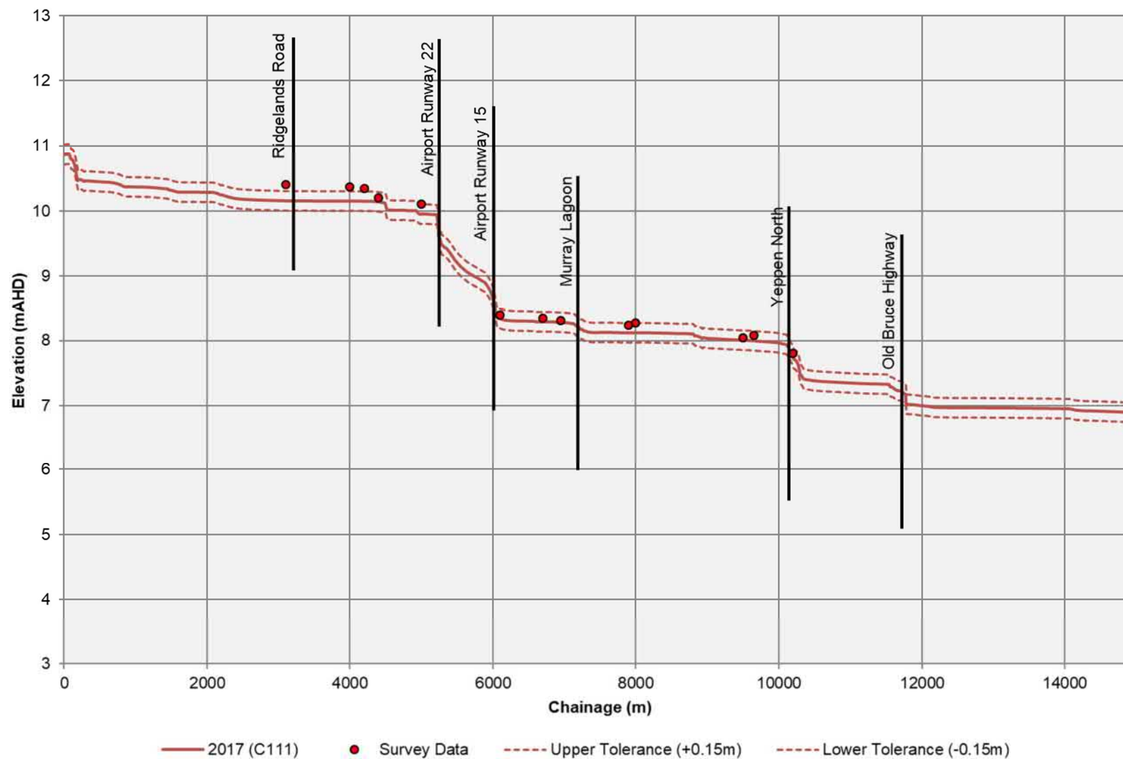
Figure 23 2017 Event Calibration – Long section Along Western Floodplain
