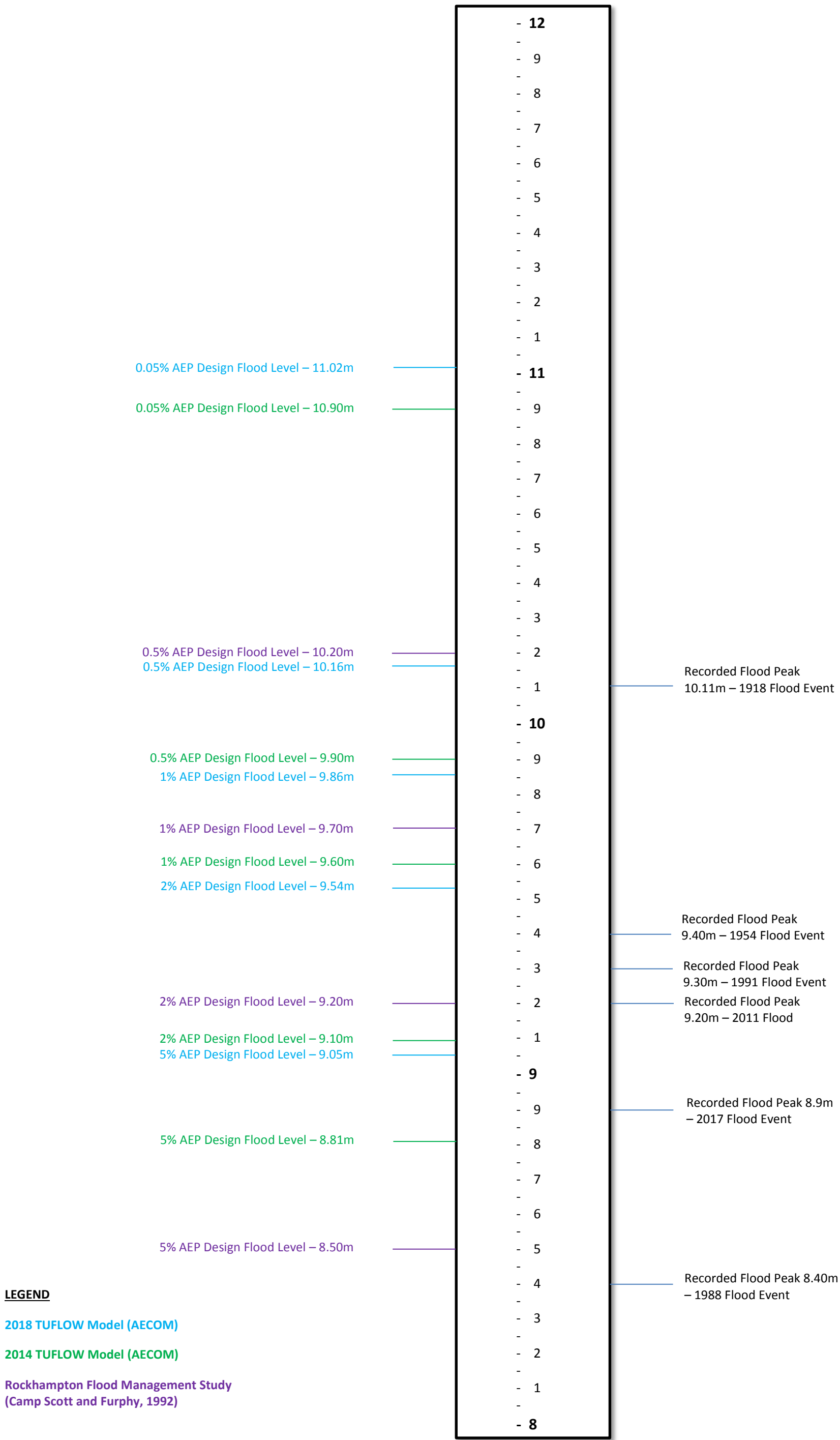
Figure 49 -Comparison of Flood Levels at the Rockhampton Flood Gauge (all levels in Gauge Datum (AHD + 1.448m)
