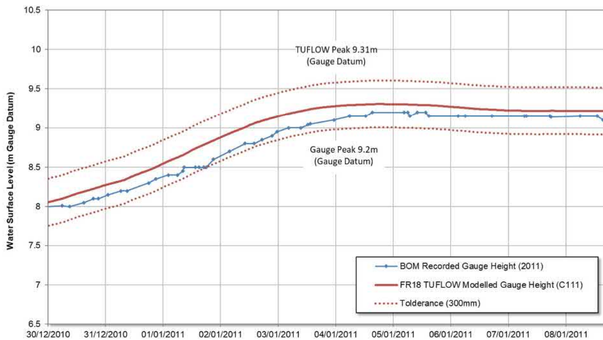
Figure 32 2011 Event Validation – Rockhampton Flood Gauge Comparison
