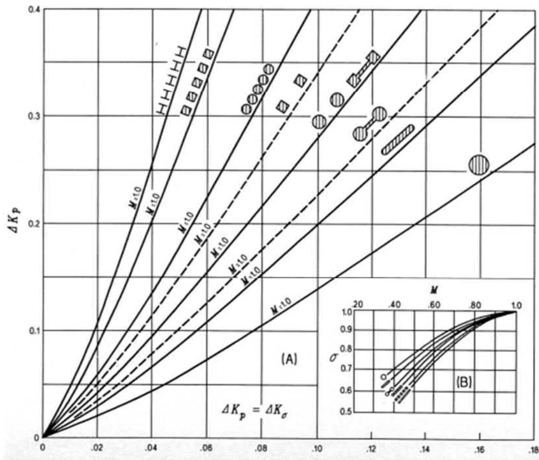
Figure 17 Incremental Backwater Coefficient for Piers (Figure 7 from Hydraulics of Bridge and Waterways, 1978)
