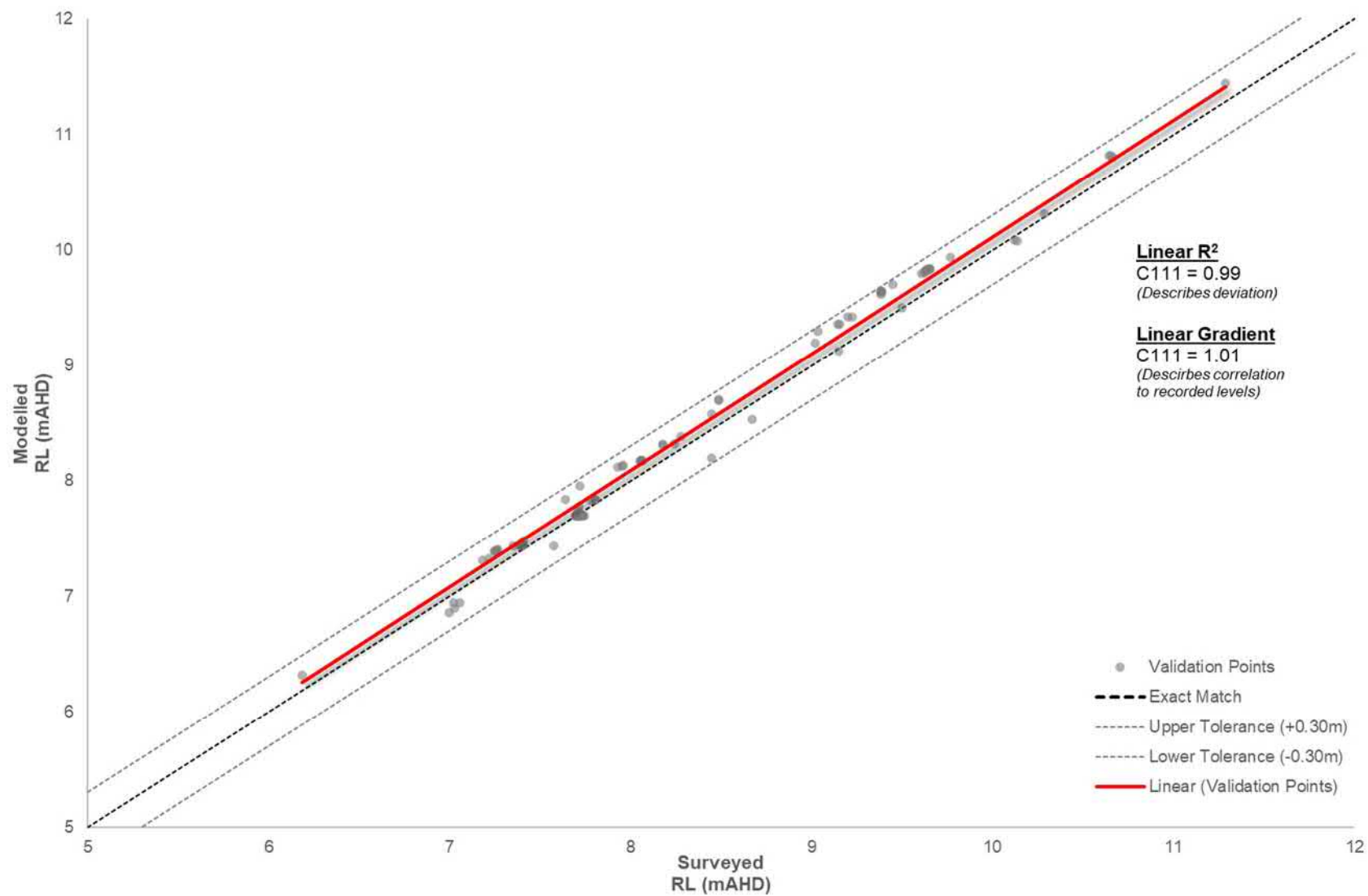
Figure 35 2011 Event Calibration Scatter Plot
