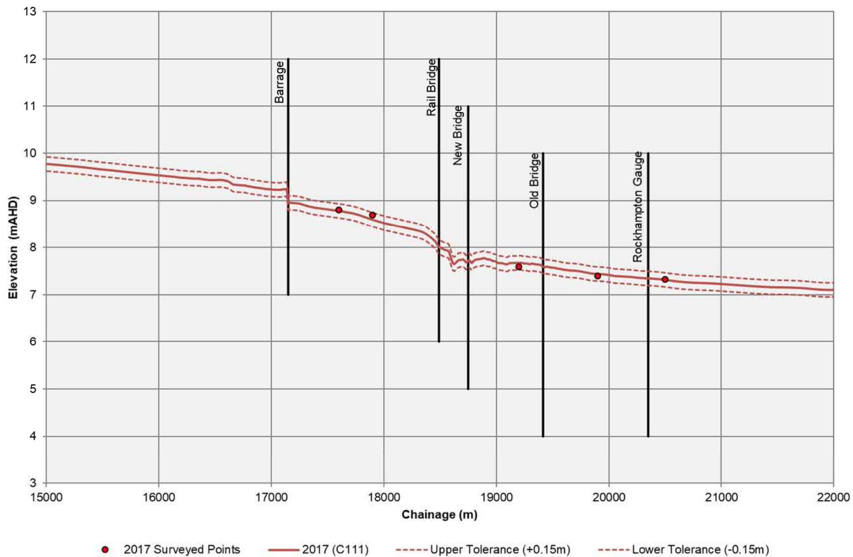
Figure 22 2017 Event Calibration – Long section Along Main River Channel
