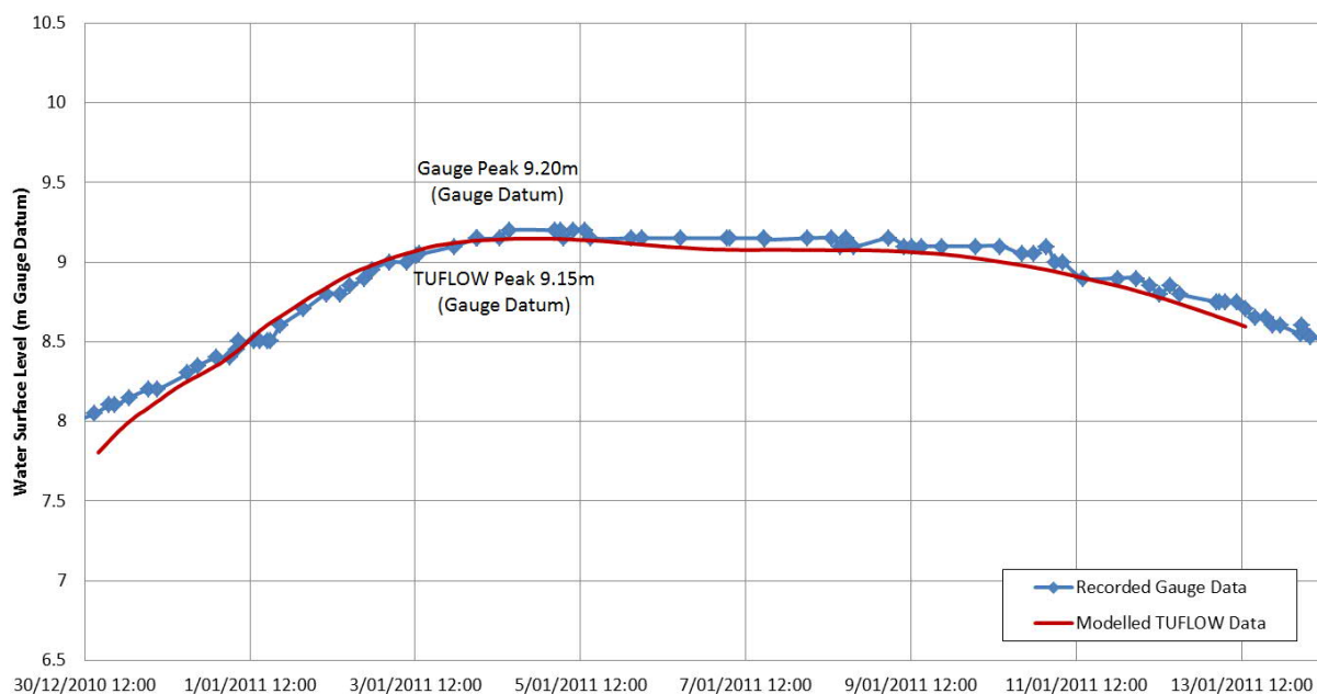
Figure 33 SRFL Rockhampton Flood Gauge Comparison – 2011 Event (source: AECOM, 2014)
