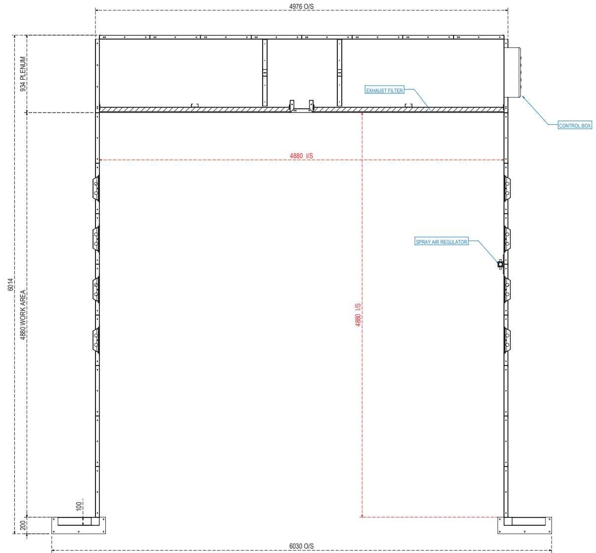
SECTION CN-CN SCALE 1:30
