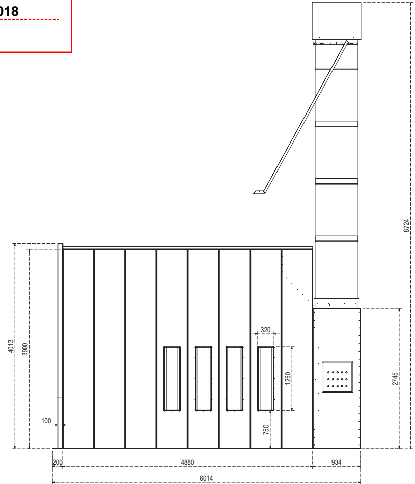
RIGHT VIEW
