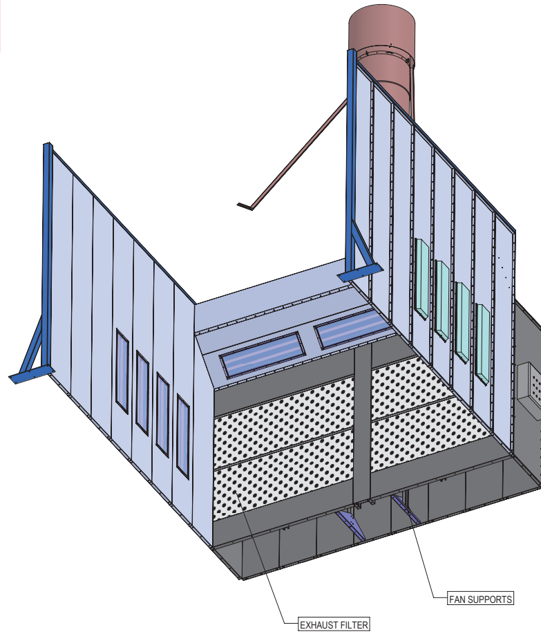
ISOMETRIC VIEW
