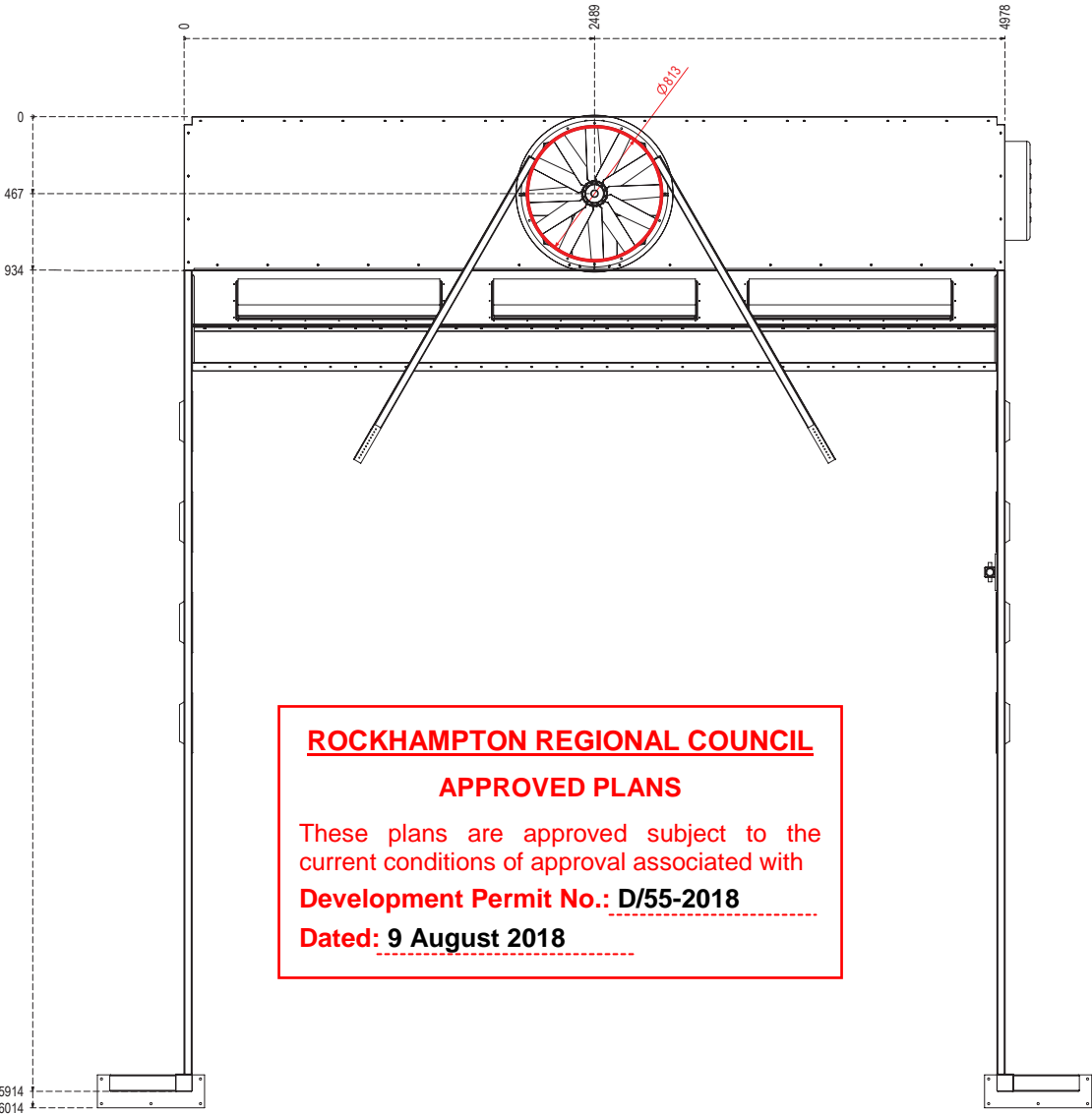
TOP VIEW
