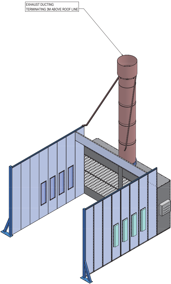
ISOMETRIC VIEW
