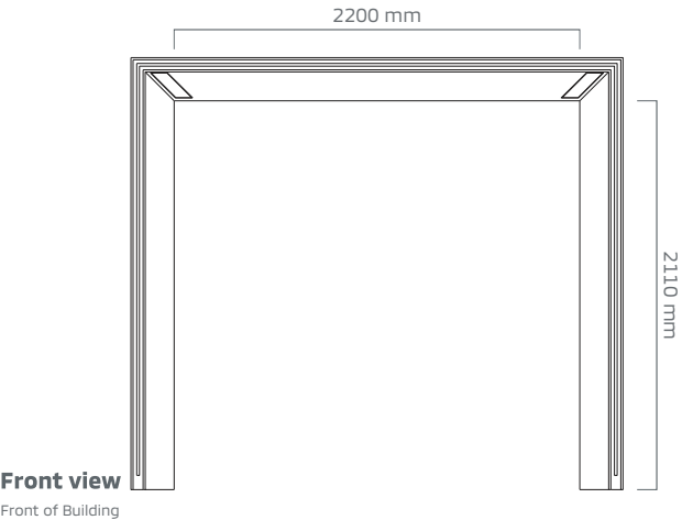
SIGN 5 ENTRY PORTAL PARTLY ILLUMINATED WITH THIN RED STRIP
